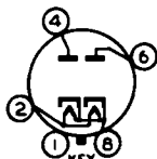
BOTTOM VIEW (5L)
